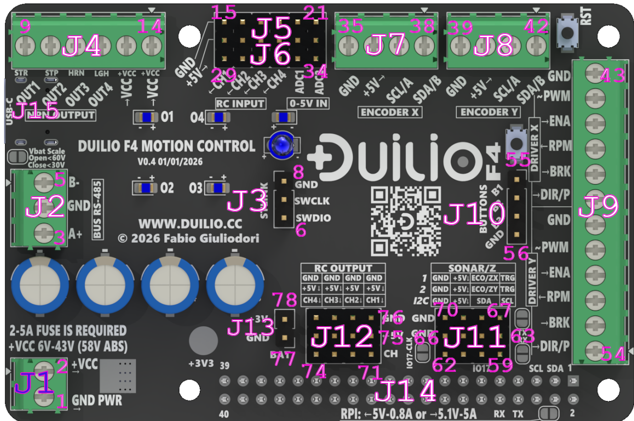
Figure 3: DUILIO F4 – Connector and pinout reference
