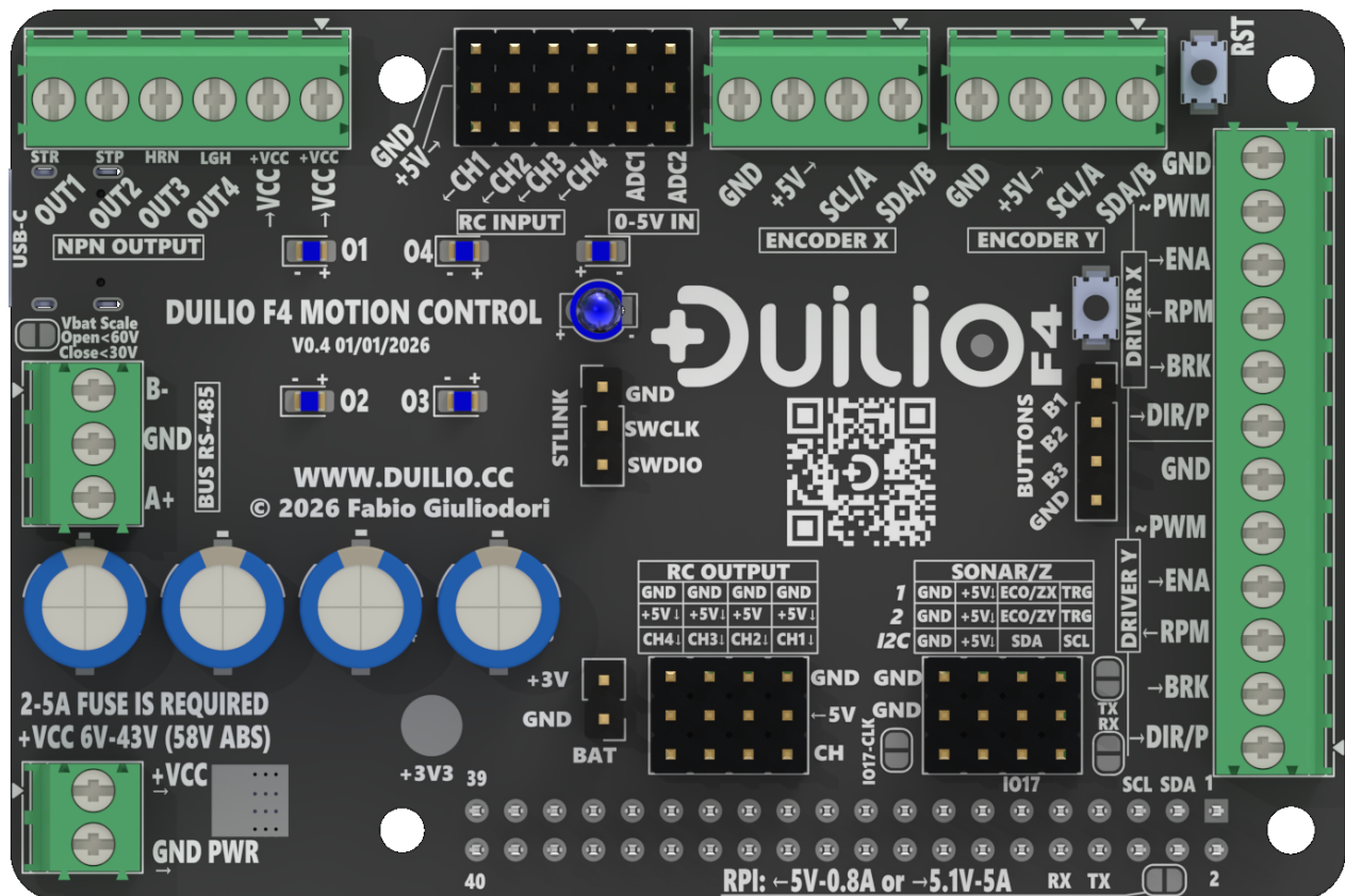
Figure 1: DUILIO F4 – Top view
