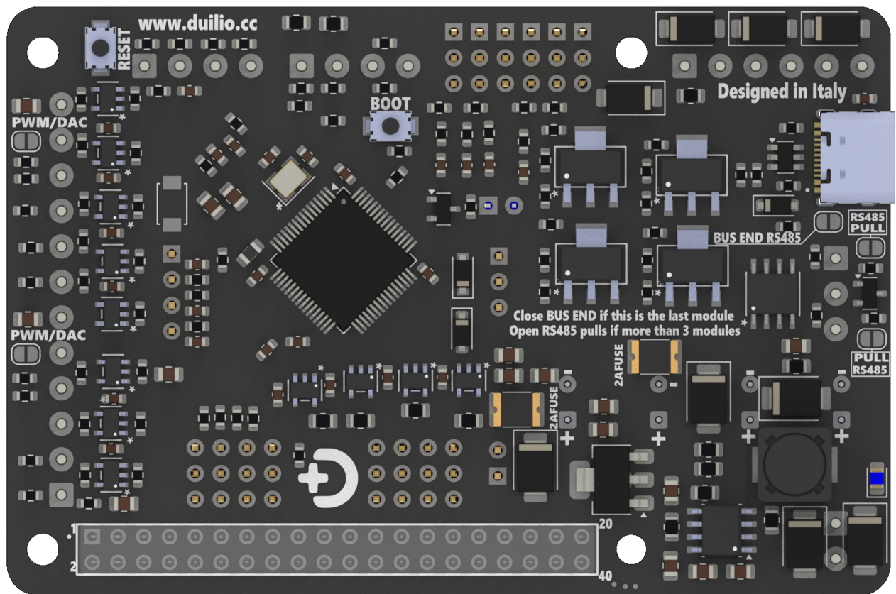
Figure 2: DUILIO F4 - Bottom view
